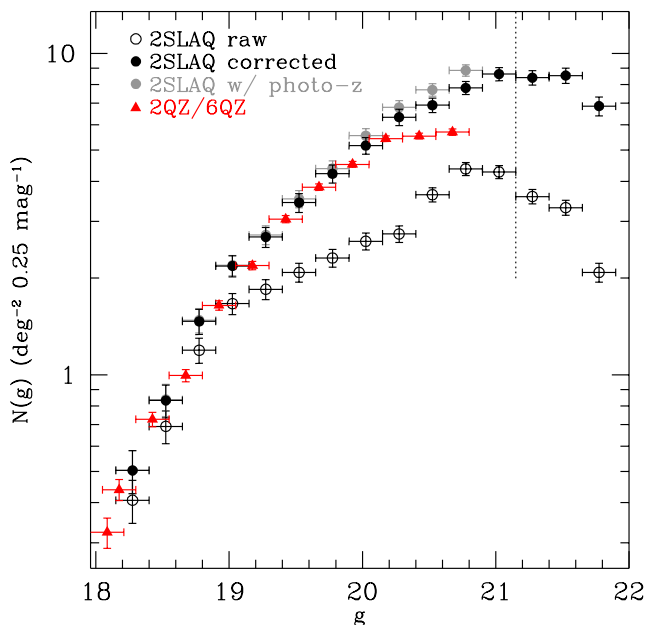
Figure 9. 2SLAQ number counts ( black circles ) compared to 2QZ number counts ( red filled triangles ) from Croom et al. (2004). The 2SLAQ number counts are given both as raw (i.e. observed; open circles ) and corrected ( filled circles ) number counts. 2SLAQ number counts are also given (as grey circles) after including photometrically identified quasars (with photometric redshifts) from Richards et al. (2004). Quasars are restricted to those with M_g < -22.5 and 0.4 < z < 2.1 (3889 quasars) for comparison with the 2QZ number counts. The dotted vertical line marks the dividing line between the 2SLAQ bright and faint samples.
